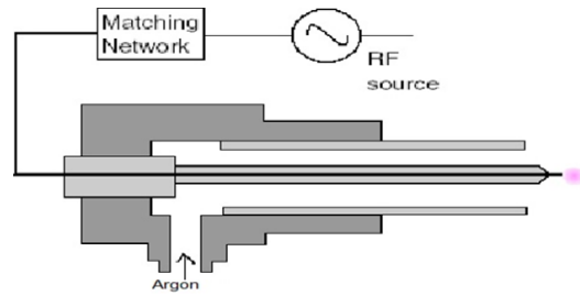
Fig. (1) Schematic diagram of the plasma needle
