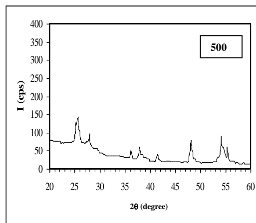
Fig. (2): The XRD pattern of TiO 2 powder annealed at 500 °C.
