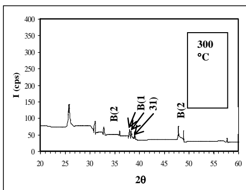
Fig. (1): The XRD pattern of TiO 2 powder annealed at 300 °C.
