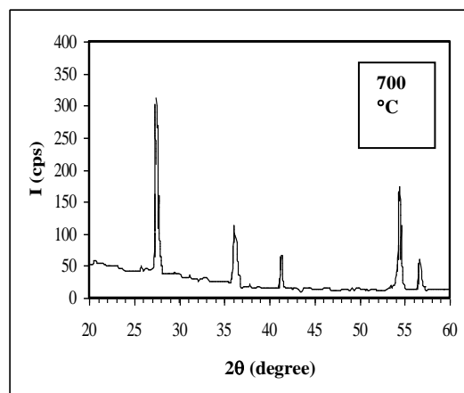
Fig. (3): The XRD pattern of TiO 2 powder annealed at 700 °C.
