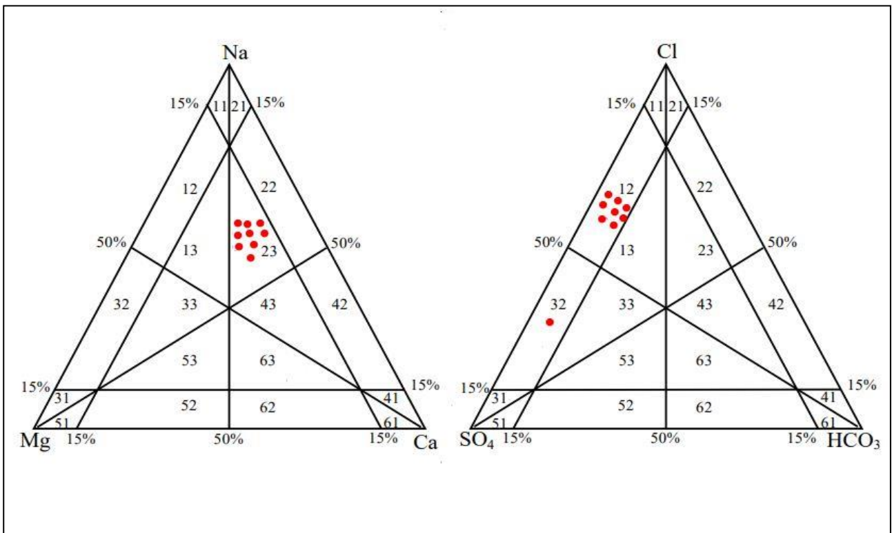
Figure 15. Distribution of Euphrates River water samples in the study area to classify their quality according to the Schuller-Solen method 1981
