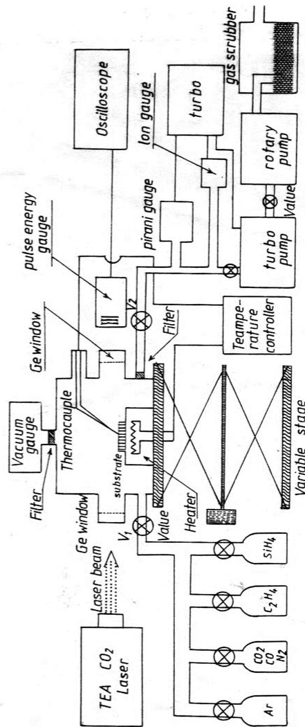
Fig.(1) Block diagram deposition system
