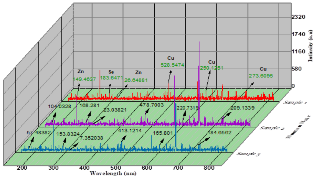
Figure 5. Shows 3D plot spectra of LIBS measurements.
