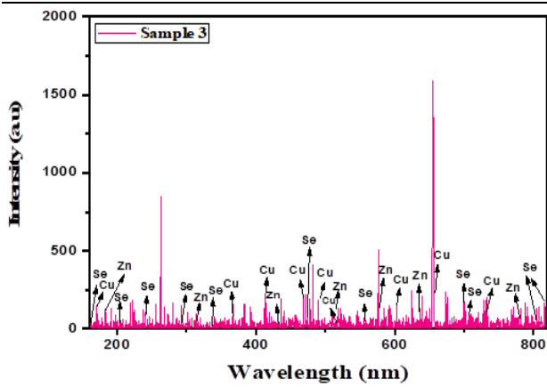
Figure 4. Shows LIBS spectra of Hypothyroidism hair fiber of sample 3
