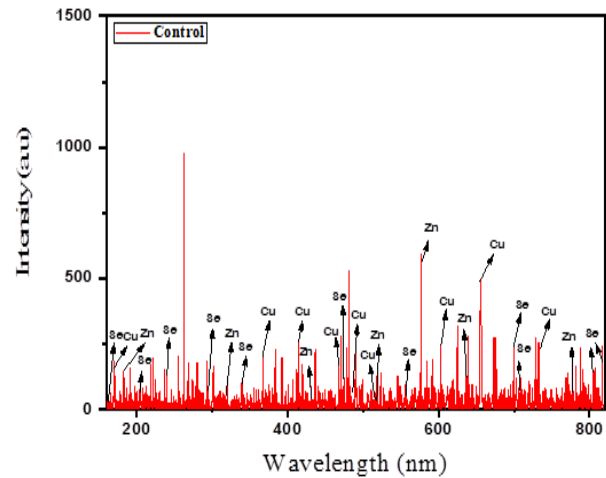
Figure 2. Shows LIBS spectra of Control hair fiber of sample 1
