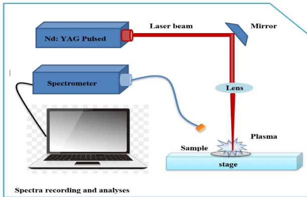
Figure 1. Shows represent LIBS Setup
