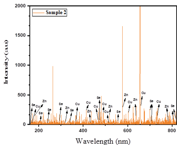
Figure 3. Shows LIBS spectra of Hypothyroidism hair fiber of sample 2
