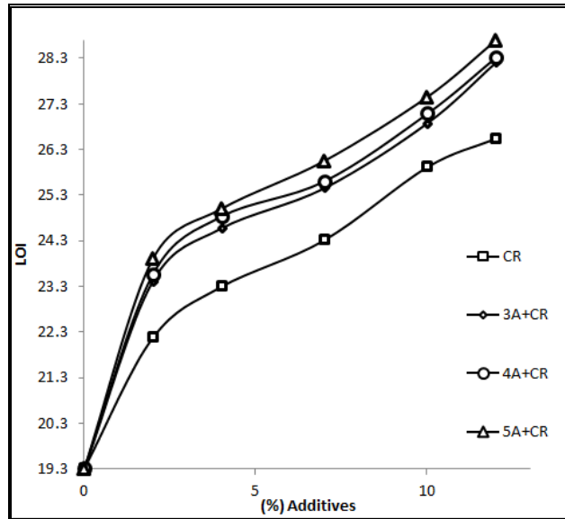
Fig. (1) LOI of the epoxy resin with additives.
