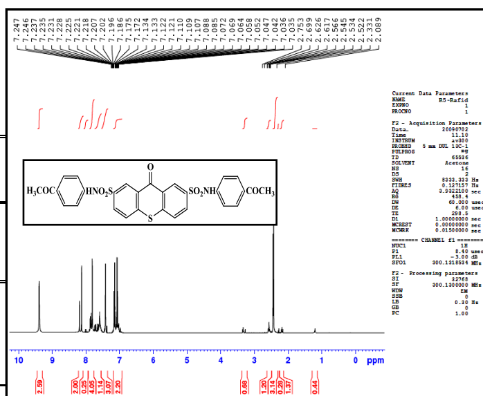
4 Fig.(7): 1 H-NMR spectrum for compound (13) 3 3
