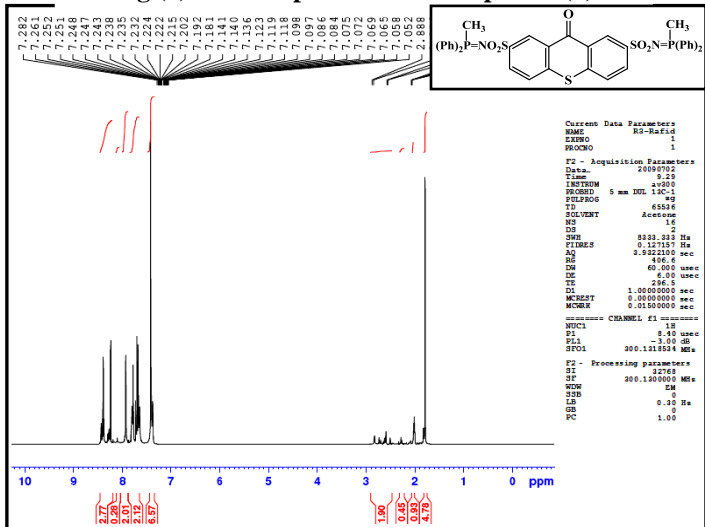
Fig.(5): 1 H-NMR spectrum for compound (6)
