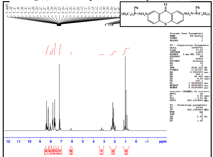
Fig.(6): 1 H-NMR spectrum for compound (8)
