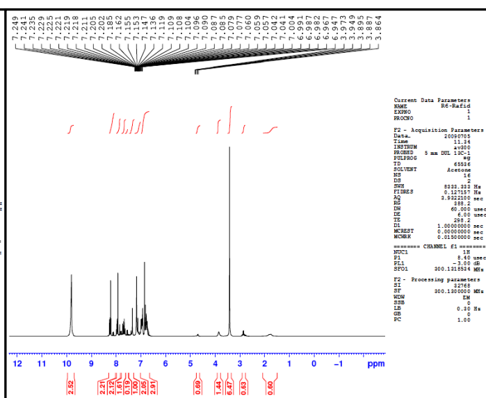
Fig.(8): 1 H-NMR spectrum for compound (14)
