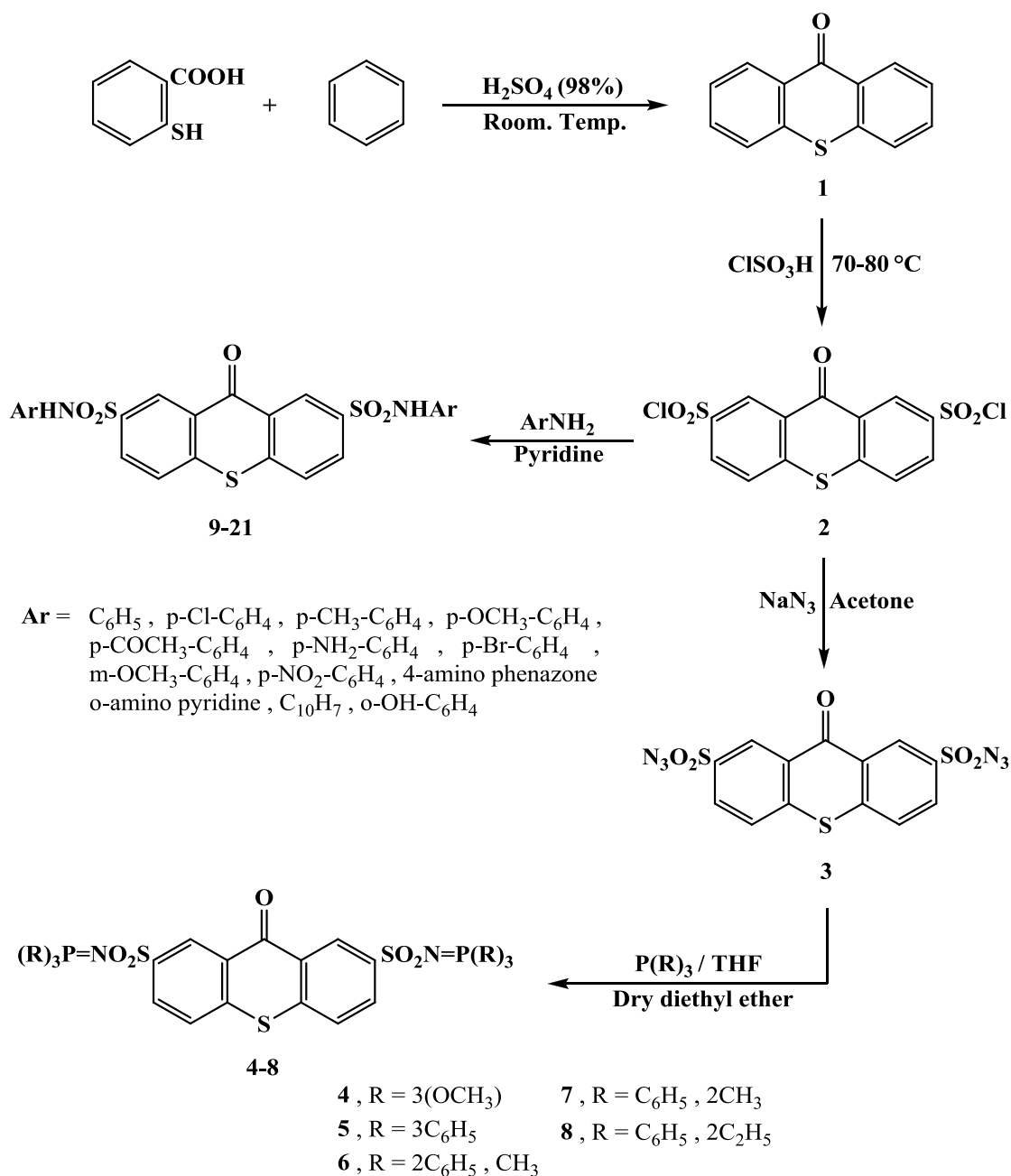
Scheme: Synthesis of thioxanthone derivatives.
