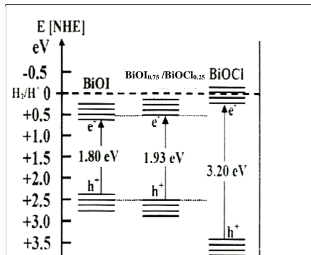
Scheme 1. Band gap structures and photo-sensitization phenomenon
