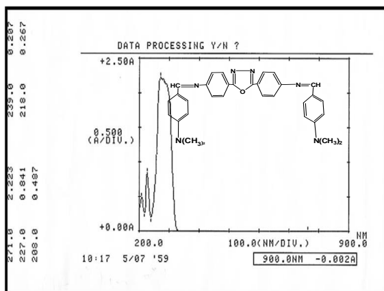
Fig. (8): U.V. Spectrum of compound (5)
