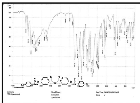
Fig. (3): FT-IR of compound (3)
