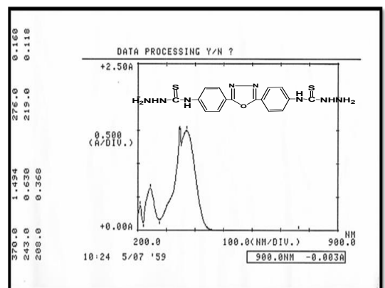
Fig. (6): U.V Spectrum of compound (1)
