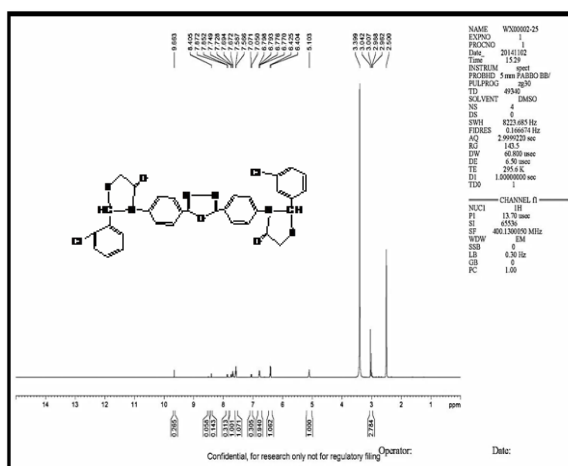
Fig. (12): HNMR of compound [10]
