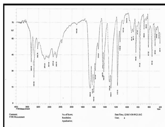
Fig. (1): FT-IR of compound (1)
