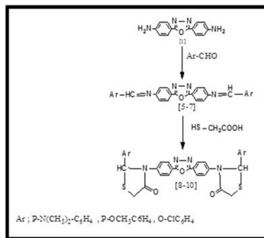
Scheme (3) Mechanism preparation of compound (5-7) and compound (8-10)
