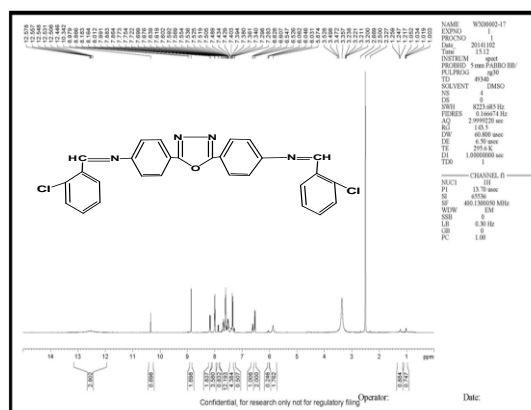
Fig. (10): HNMR of compound (6)
