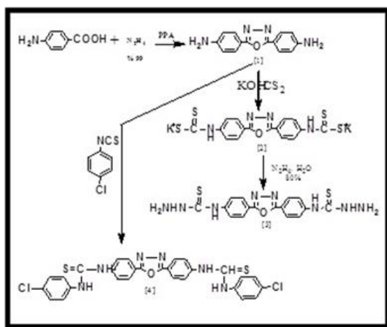
Scheme (1) Mechanism preparation of comp.(1-4)
