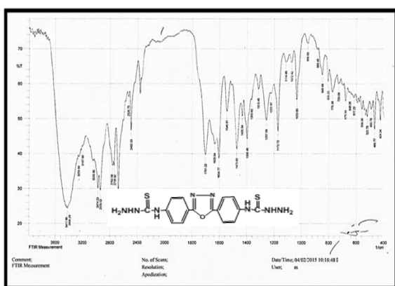
Fig. (2): FT-IR of compound (2)
