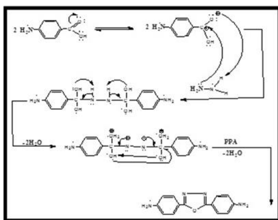
Scheme (2) Mechanism preparation of compound (1)
