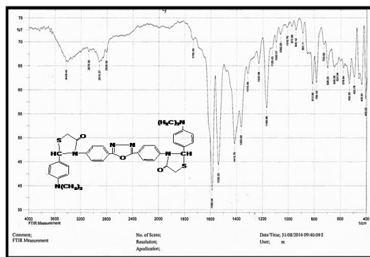
Fig. (5): FT-IR of compound (8)
