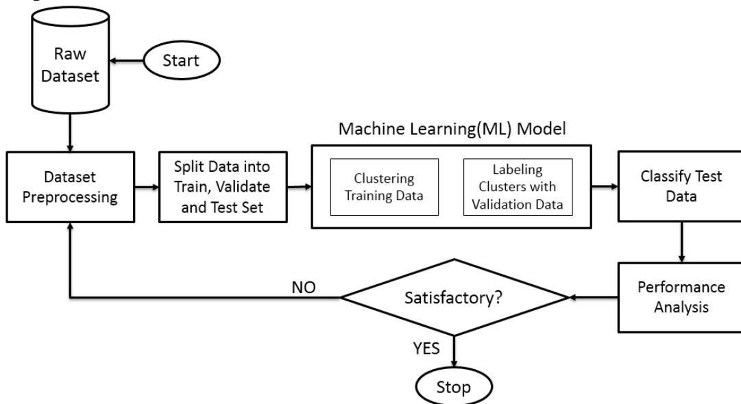
Figure 1. The proposed semi-supervised learning architecture to prevent BHP flood attack
