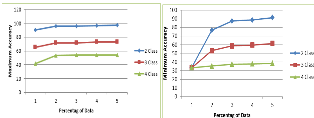
Figure 5. Maximum(left) and minimum(right) accuracy of the model
