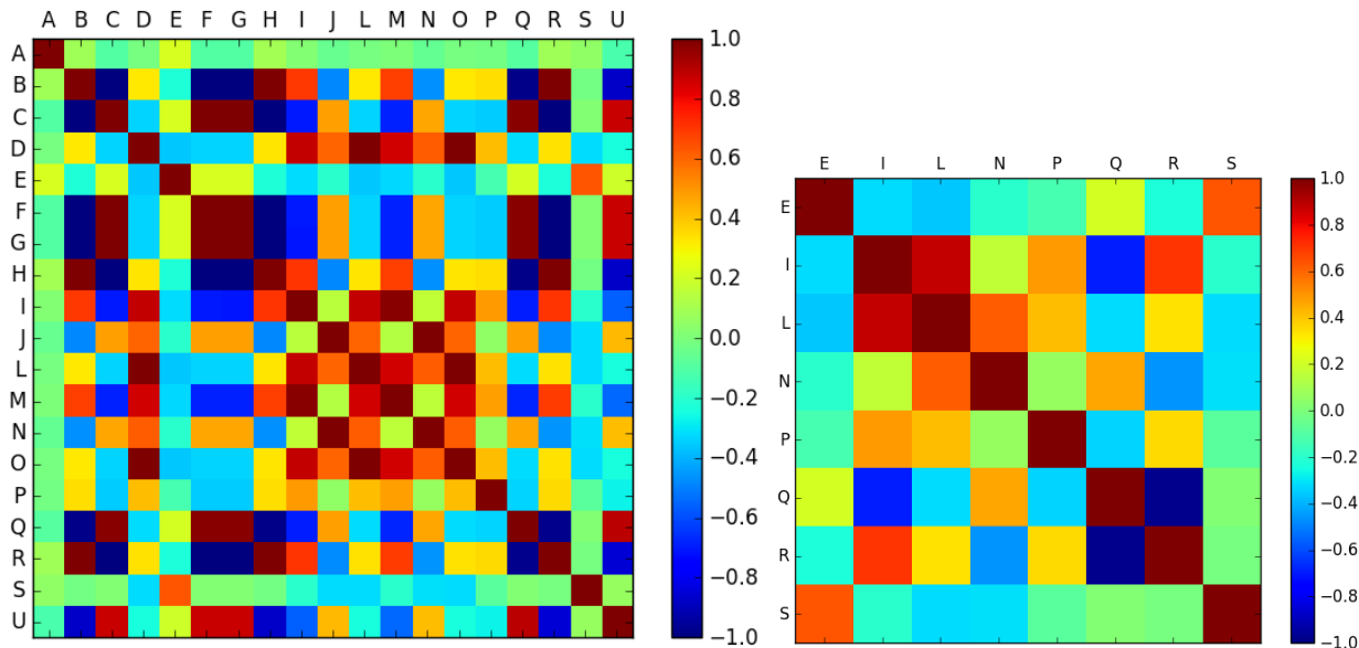
Figure 2. Correlation heatmap of the dataset before (left) and after (right) feature selection
