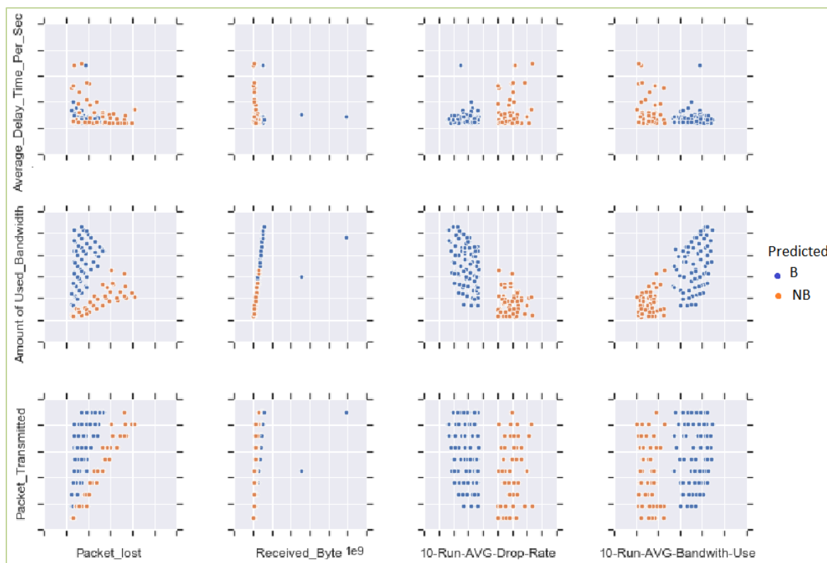
Figure 4. Plot of predicted labels for the test dataset
