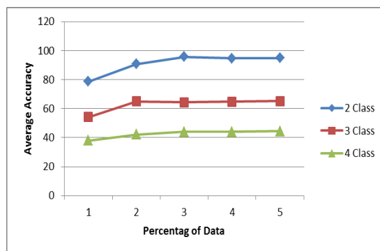
Figure 6. Average accuracy of the model
