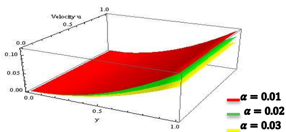
Figure 2. velocity surface for (\alpha = 0.01, 0.02, 0.03) when keeping \phi, \lambda_1, t, \lambda_2, \lambda_3, N, \beta , fixed
