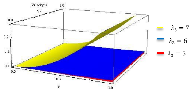
Figure 5. velocity surface for (\lambda_3 = 7, 6, 5) when keeping \alpha, \phi, \lambda_1, \beta, t, \lambda_2, N , fixed
