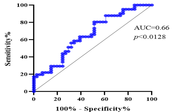
Figure 10D. The ROC curve of Zn for the detection of CRC.
