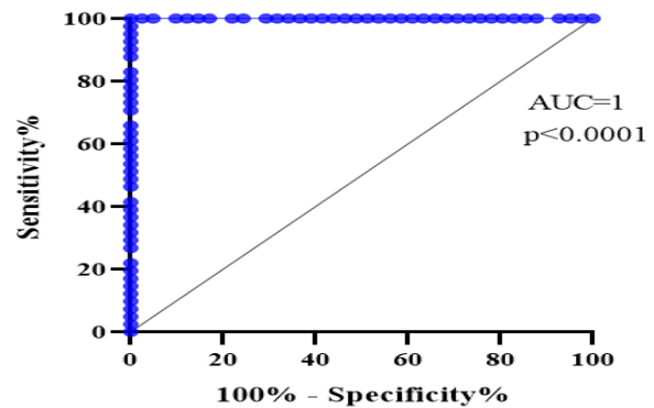
Figure 8B. The ROC curve of CEA for the detection of CRC.
