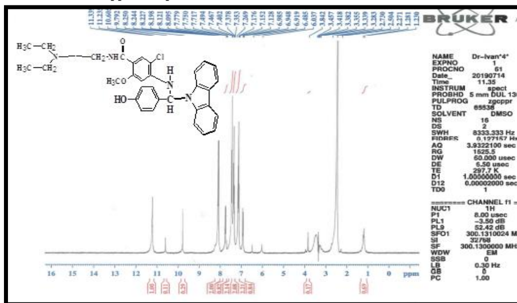
Figure 3. The results of ( ^1\text{H} -NMR) spectral for synthesized materials (A)
