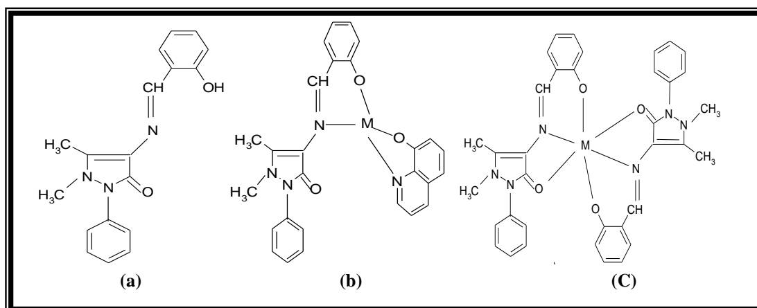
(Fig 1)The suggests Structure (a) Ligand(HL) Schiff base ,(b) [\text{M}(\text{L})(\text{Q})] complexes with (\text{M}=\text{Zn}(\text{II}),\text{Cd}(\text{II}) and \text{Hg}(\text{II})) ,(c) [\text{M}(\text{L})_2] complexes (\text{M}=\text{Mn}(\text{II}) and \text{Fe}(\text{II}))
