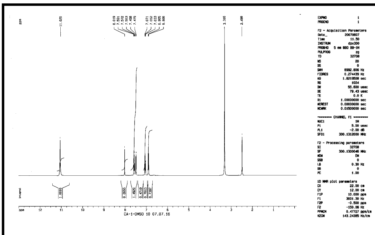
Fig. 2 1 H-NMR spectrum of compound 10
