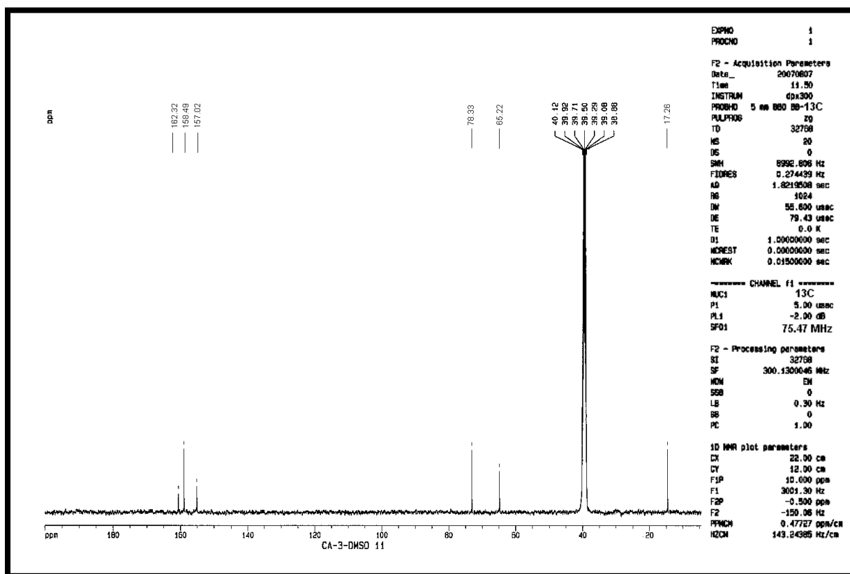
Fig. 1 13 C-NMR spectrum of compound 4
