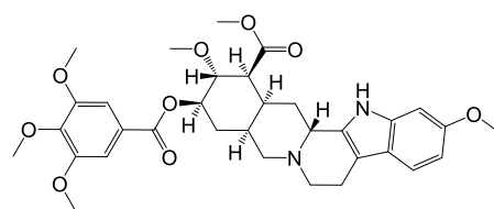
Reserpine (9)
