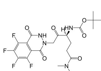
N,N-Dimethylglutamine (49)
