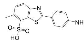
MAC-8120 (3)
