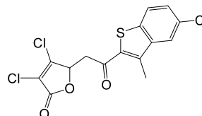
MAC-30731 (6)
