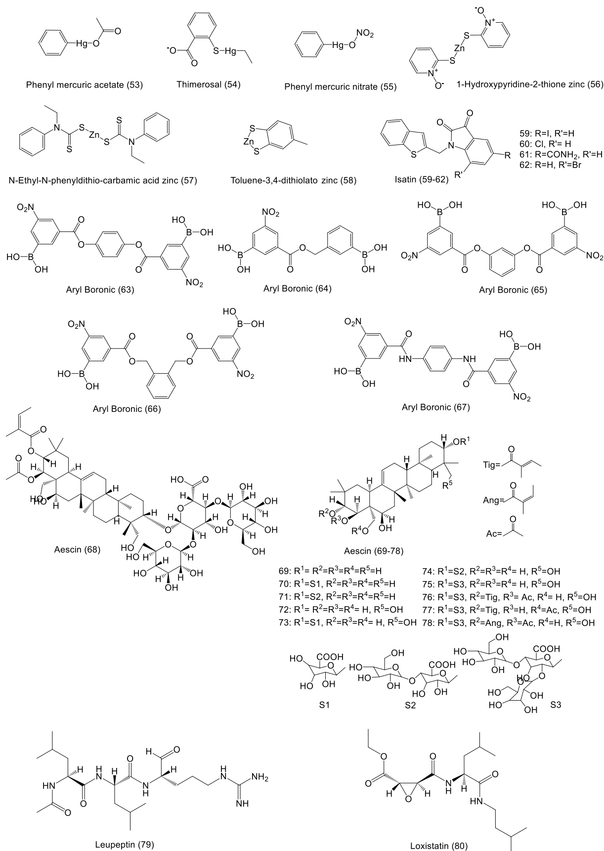
Figure 1. Chemical compositions of natural compounds and drugs tested against M Pro of SARS and MERS-CoV
