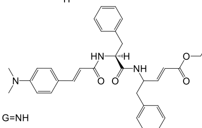
unsaturated ester (27)
