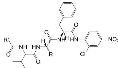
Tripeptide anilide (35-41)
