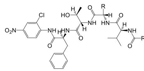
Tetrapeptide anilide (42-48)
