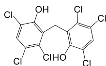
Hexachlorophene (8)
