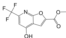
MAC-13985 (4)
