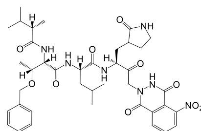
Keto-glutamine (50)
