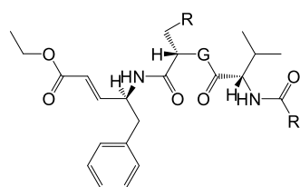
AG7088 (19-22), G=CH 2 AG7088 (23-26), G=NH
