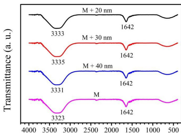
Fig. 11. FTIR spectra of the interaction between Ag NPs and the Methomyl (M) pesticide.
