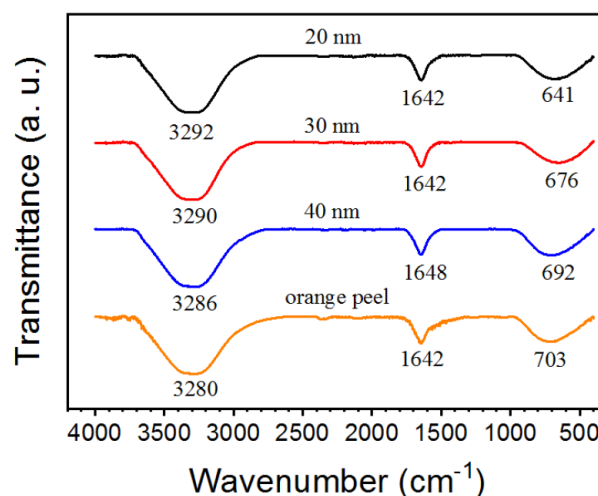
Fig. 7. FTIR spectra of orange peel extract and fabricated Ag NPs.
