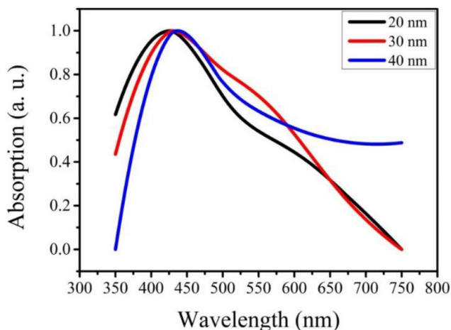
Fig. 4. UV-VIS spectra of fabricated nanoparticles.
