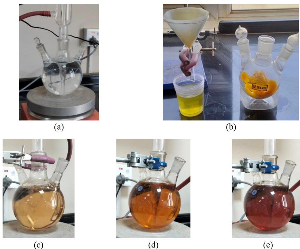
Fig. 2. Identifying the formation of nanoparticles through a visual representation of the green synthesis of Ag NPs from (a) Orange peel extract and (b) Silver nitride solution, (c) 0.5 M, (d) 1 M, and (e) 2 M silver nitride concentrations.
