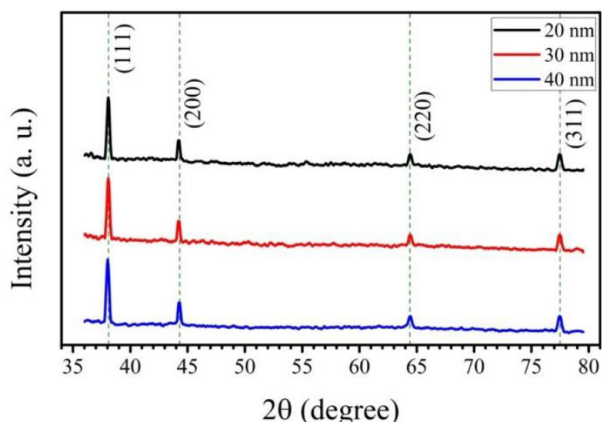
Fig. 6. XRD pattern of fabricated nanoparticles.
