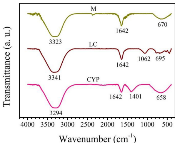
Fig. 8. FTIR spectra of the pesticides Cypermethrin (CYP), Lambda-cyhalothrin (LC), and Methomyl (M).
