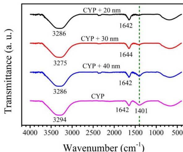
Fig. 9. FTIR spectra of the interaction between Ag NPs and the Cypermethrin (CYP) pesticide.
