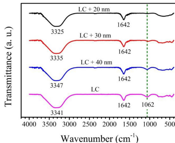
Fig. 10. FTIR spectra of the interaction between Ag NPs and the Lambda-cyhalothrin (LC) pesticide.
