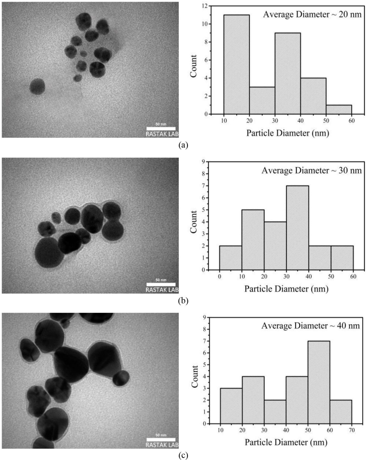
Fig. 3. TEM images and associated histograms of (a) 20 nm, (b) 30 nm, and (c) 40 nm Ag NPs.
