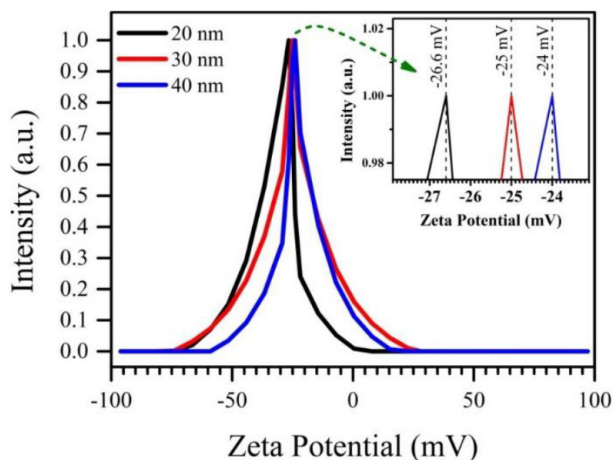
Fig. 5. Zeta potential of fabricated nanoparticles.
