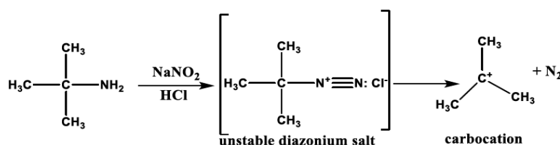
Scheme 1. azo coupling reactions
