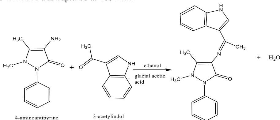
Figure 1. Synthesis of Schiff base ligand (L)
