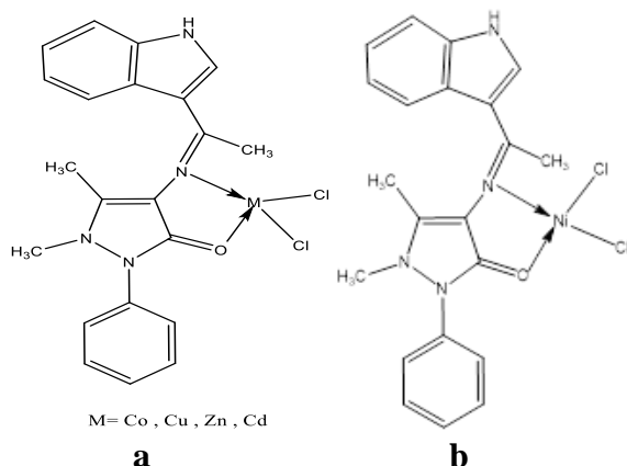
Figure 6. The structure of the prepared complexes a [M(L)Cl 2 ] b [Ni(L)Cl 2 ]
