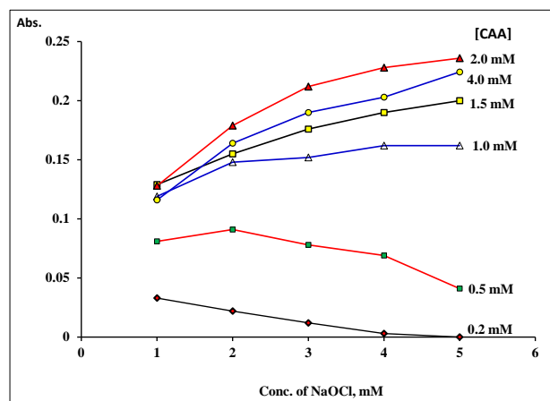
Figure 4. Effect of changing CAA and NaOCl concentrations. [mebendazole] = 10 \text{ mg L}^{-1} . RC1 = 40 \text{ cm} , RC2 = 60 \text{ cm} , sample volume 60 \mu\text{L} , total flow rate = 1.8 \text{ mL/min} , wavelength = 530 \text{ nm} .
